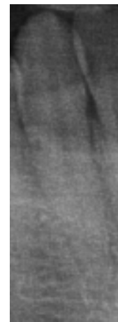
Tooth
