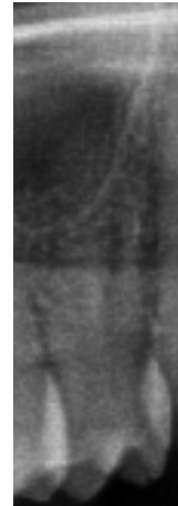
Tooth
