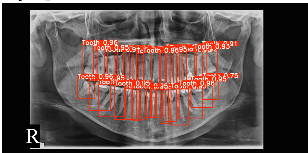
Image: train_526
