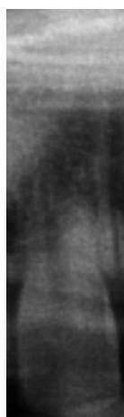
Tooth
