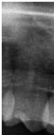
Tooth
